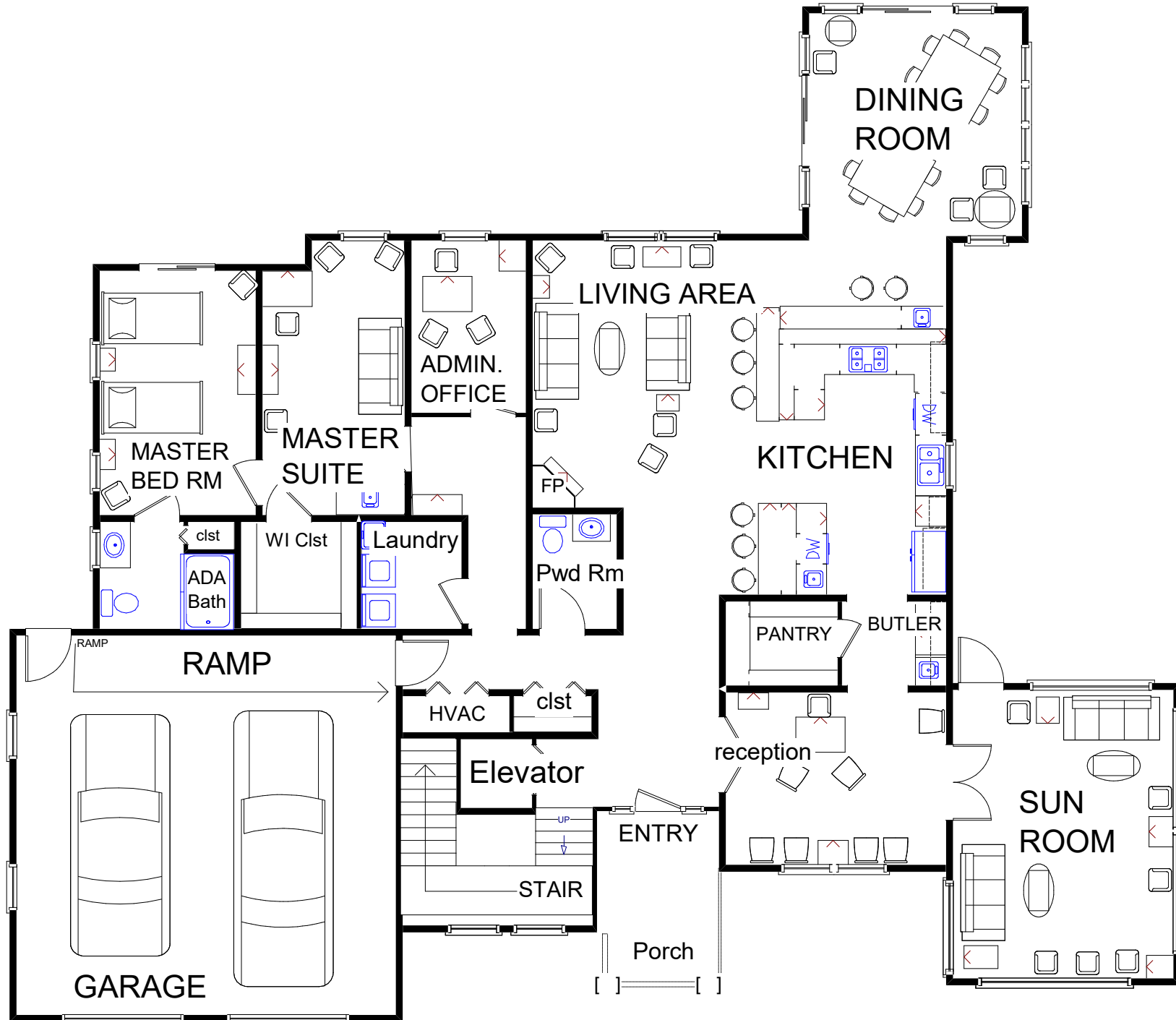
ASSISTED LIVING & SENIOR CARE & SHARE PLANS-1st FLOOR
